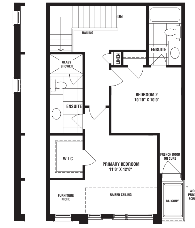
PART. OPT. 2 BEDROOM THIRD FLOOR PLAN ELEV. 'A' END CONDITION
