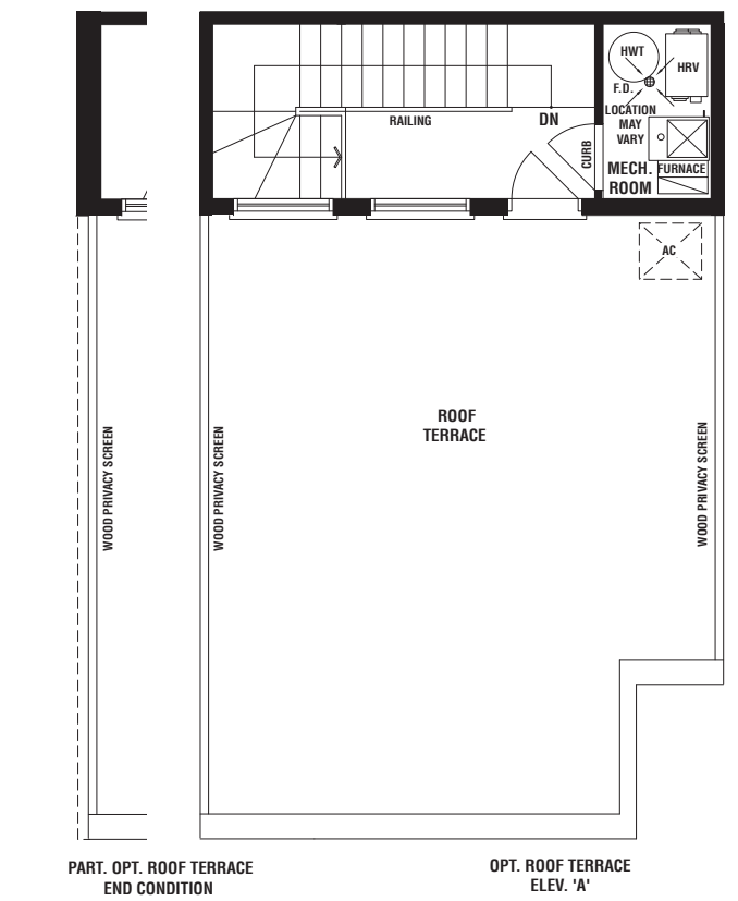
PART. OPT. ROOF TERRACE END CONDITION
