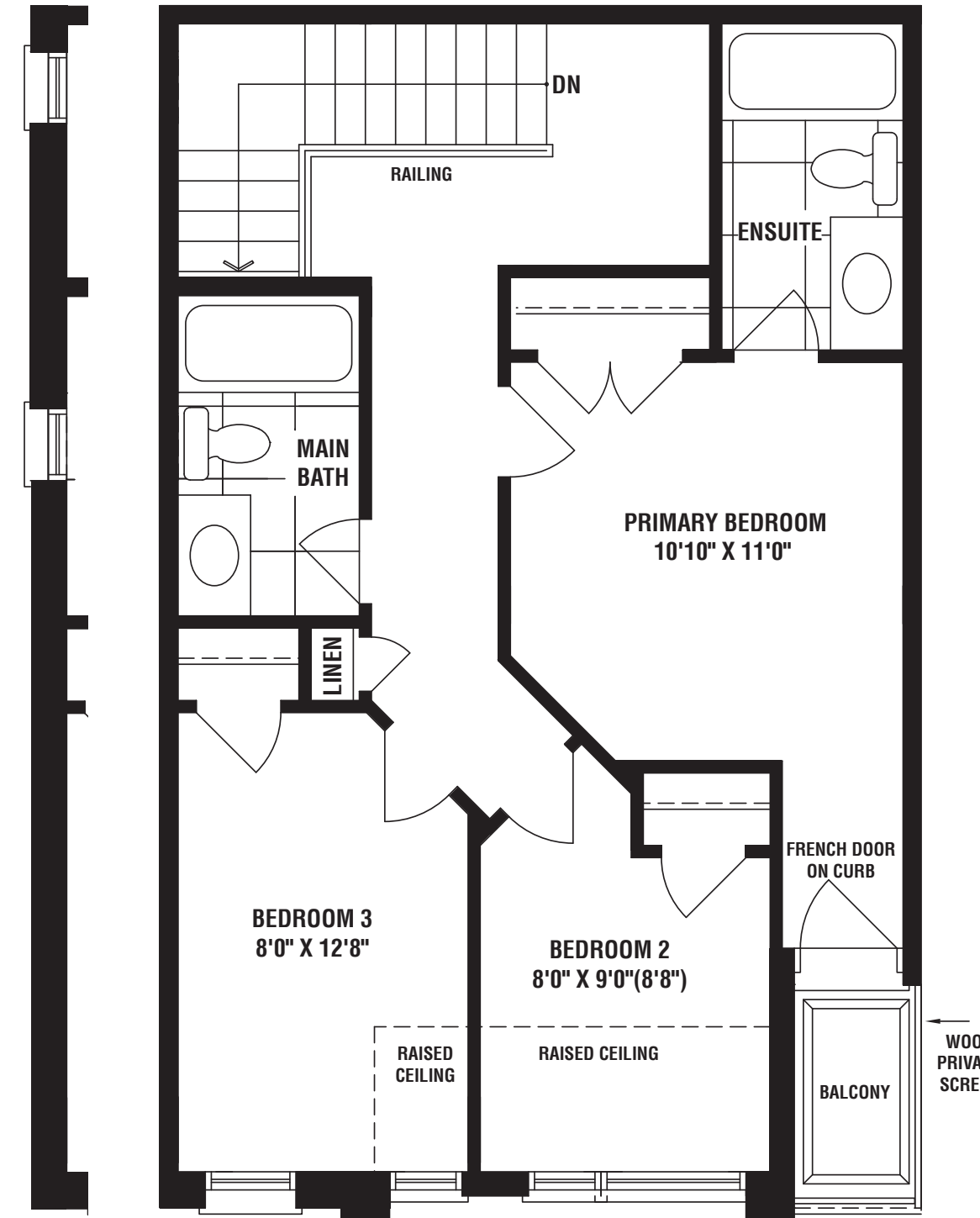
PART. THIRD FLOOR PLAN ELEV. 'A' END CONDITION
